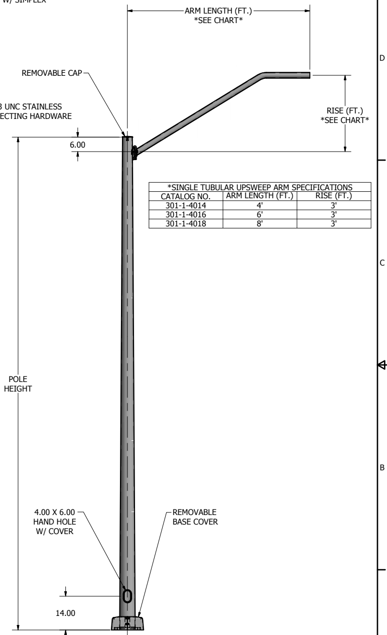
POLE DETAIL
